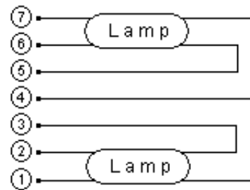
Connection diagram
